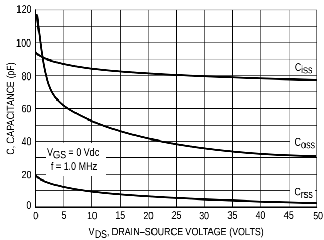
Figure 10. Capacitance versus Voltage
